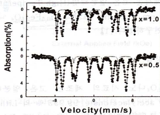
Fig. 3. \text{Tb}_{3-x}\text{Bi}_x\text{Fe}_5\text{O}_{12} 의 Mössbauer spectrum
