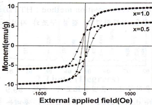
Fig. 2. \text{Tb}_{3-x}\text{Bi}_x\text{Fe}_5\text{O}_{12} 의 Hysteresis loop
