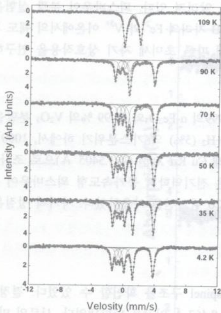
Fig. 1. The Mössbauer spectra of FeV 2 O 4 at various temperatures below TN.
