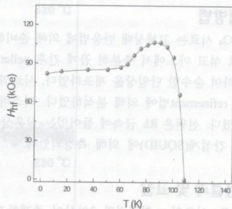
Fig. 2. Temperature dependence of the magnetic hyperfine field for FeV 2 O 4 .
