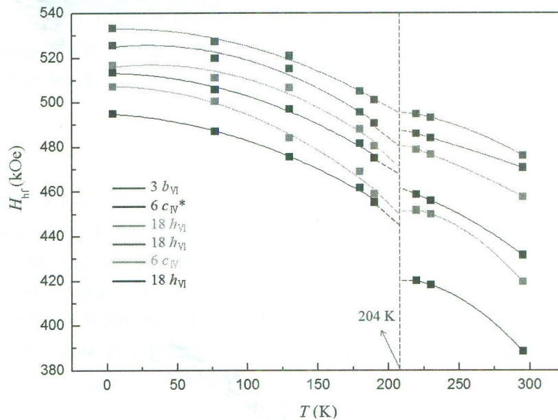
Figure 2. Temperature dependence of the magnetic hyperfine field ( H_{hf} ) of \text{Ba}_2\text{CoNiFe}_{12}\text{O}_{22} .
