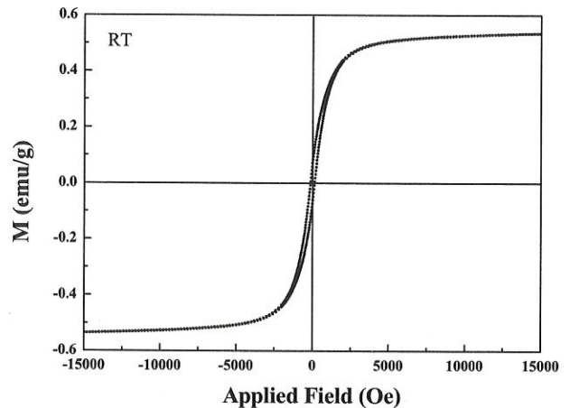
Fig.1. Hysteresis loop for \text{Fe}_2\text{O}_3 powders at 295 K.
