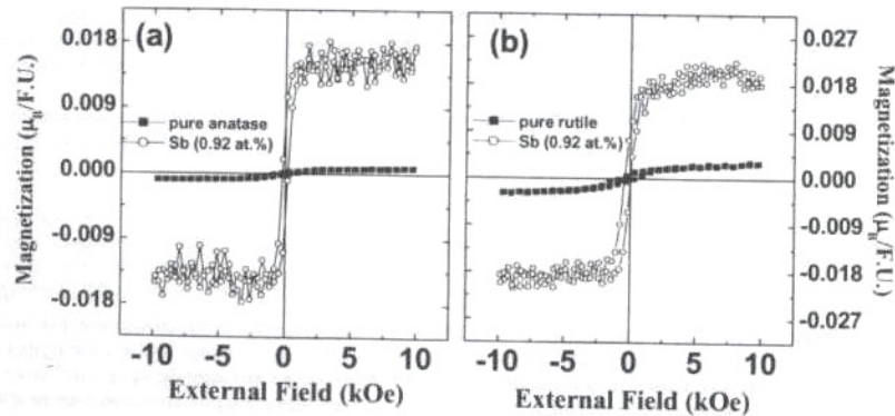
Fig. 1. Magnetic hysteresis data for pure and Sb-doped \text{TiO}_{2-x} thin films at room temperature: anatase phase (a) and rutile phase (b).
